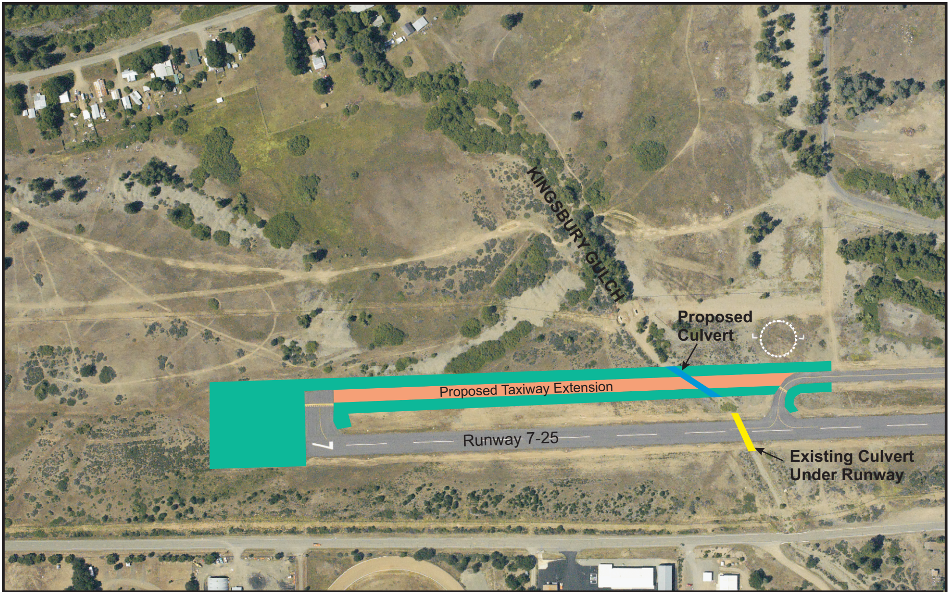
Figure 1-3 Proposed Taxiway Extension, Culvert, Runway and Taxiway Safety Area Locations
