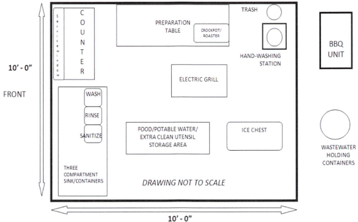
Temporary Food Facility Floor Plan Example
